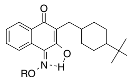
Scheme 2. The predominant Amphi conformer ( E -isomer) of 2 (R = H) and 3 (R = CH 3 ).
